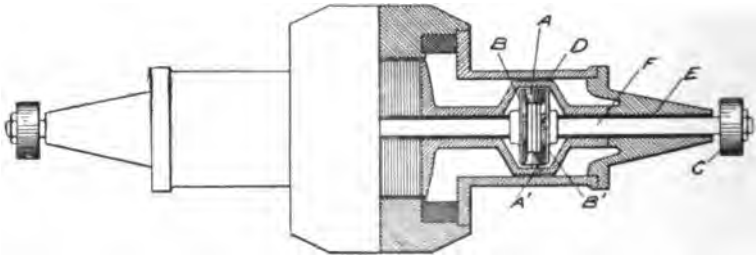
FIG. 435.—Part Sectional Diagram of a Single Motor, arranged for driving both wheels through differential gear. A and A' are the pinions of the differential gear; B, the bevel gear of the left-hand road wheel; D, bevel gear on right-hand road wheel; C, spur pinions driving internal gear on road wheels; E, sleeve on rotating shafts, F, of pinions, C and C.
